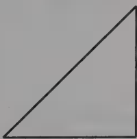
45°–45°–90°
